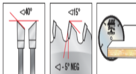
H-ATB GRIND HIGH OR ACUTE ANGLE ALTERNATE TOP BEVEL
