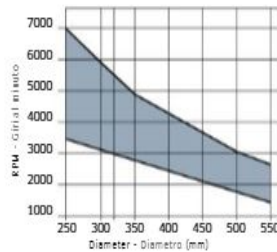
Minimum and maximum RPM based on the blade
