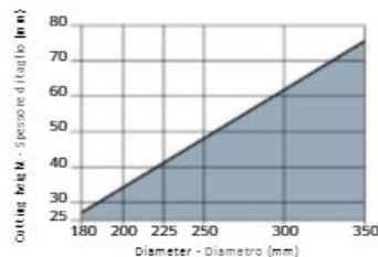
Maximum depth of cut based on the blade diameter.
