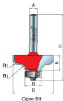
Ogee Bit
