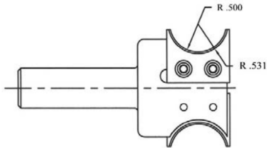
Body #8240 for material thickness of 1" - 1 1/16"
