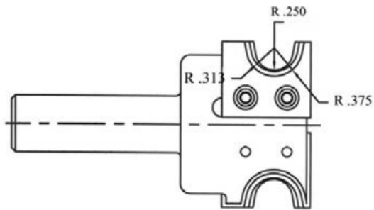
Body 8230 for material thickness of 1/2" to 3/4"
