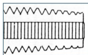
TAPER Type 23-UB, 23-UBN, 23 Type 31-UB, 31-UBN, 31 Eight to ten threads chamfered for easy thread starting in tough materials.
