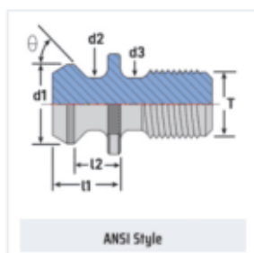
CAT Retention Knobs
