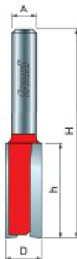
Double Flute
